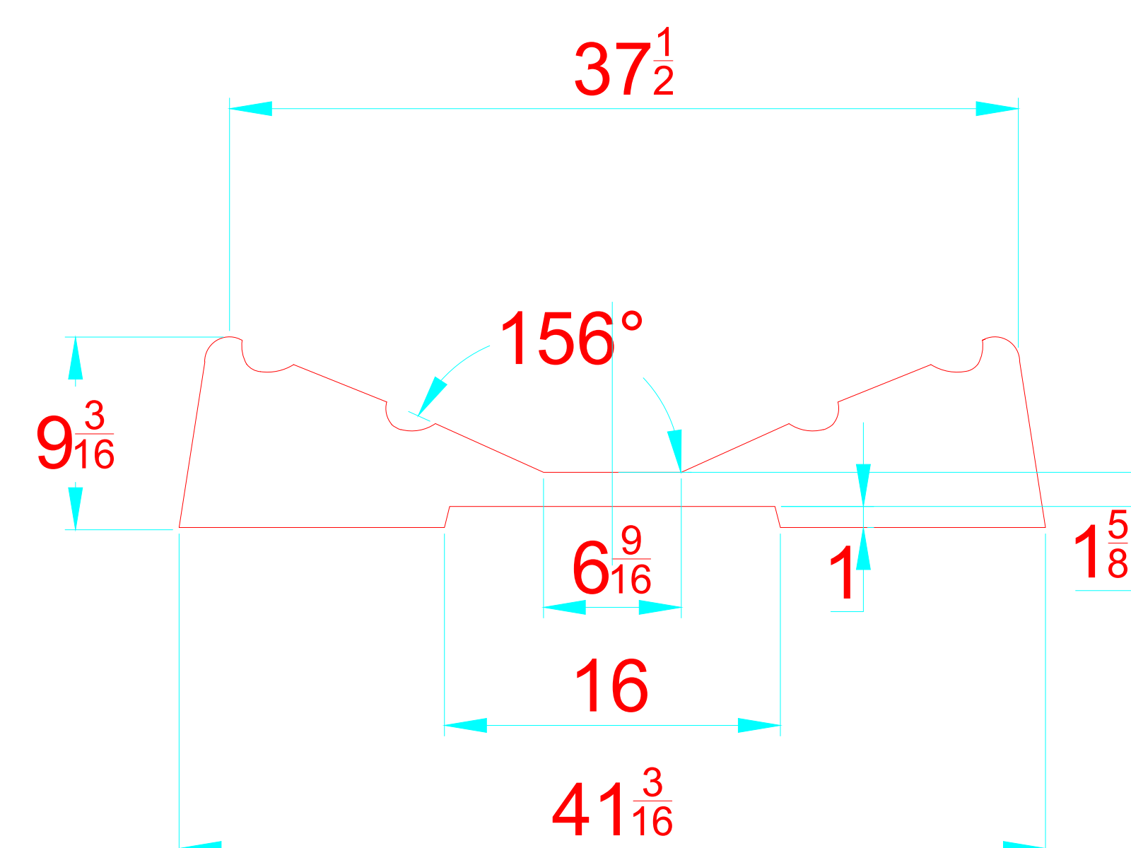
TRANSVERSAL SECTION "A" SECCION TRANSVERSAL "A"
